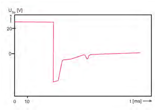
Figure 9-13 RC circuit with a suppressor diode
