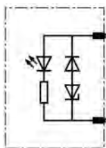
Surge suppressor, diode combination with LED
