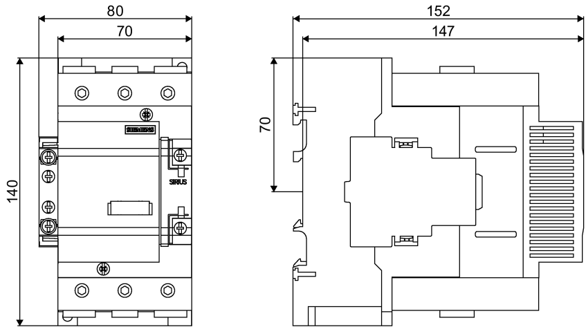
Figure C-45 3RT264.-1...capacitor contactors (size S3)
