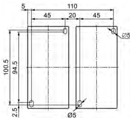
Figure C-58 Drilling diagram for 3RA233.-8XB30-1 reversing contactor assemblies
