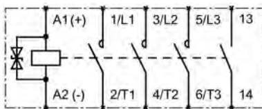
S00 contactor, with internal suppressor diode, 1 NO contact
