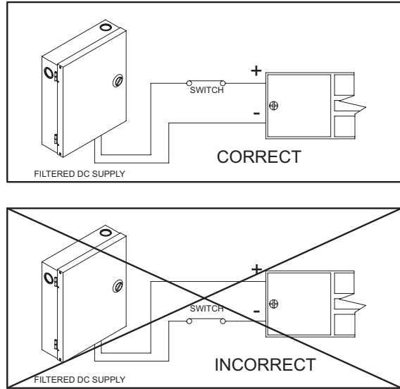
Fig. 2 – Power Connections
