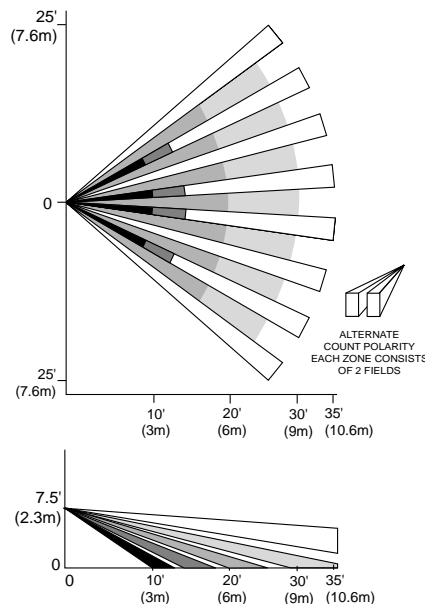
Figure 1. Protection Pattern
