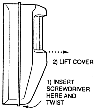
Figure 2. Cover Removal
