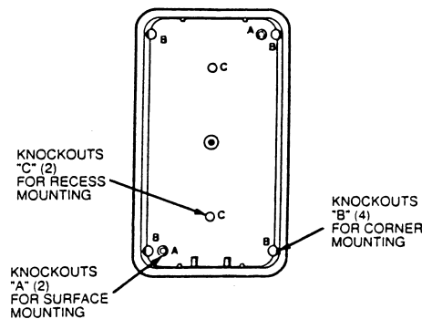
Figure 3. Mounting Holes in Base
