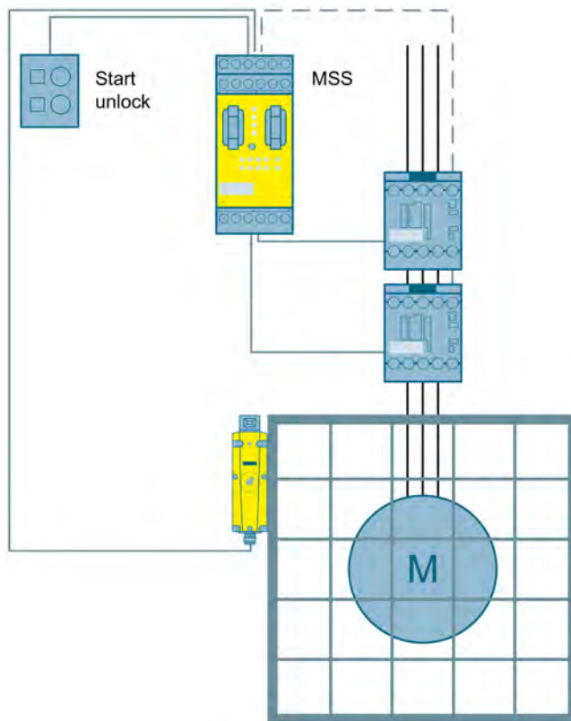
Figure 3-36 Protective door monitoring with tumbler to SIL 2 or PL d with a Modular Safety System
