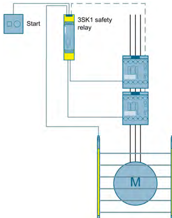
Figure 3-37 Access monitoring using a light curtain to SIL 3 or PL e with a 3SK1 safety relay
