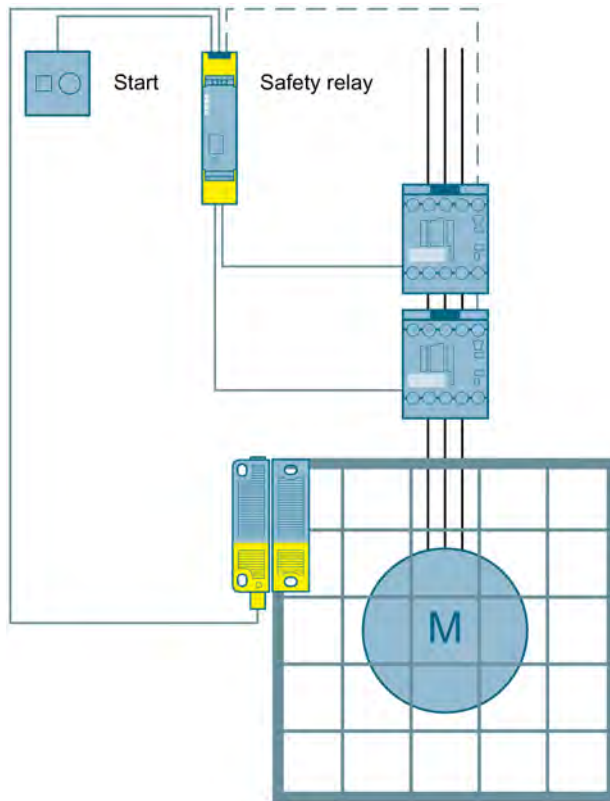
Figure 3-32 Protective door monitoring by means of RFID switch to SIL 3 or PL e with a 3SK1 safety relay
