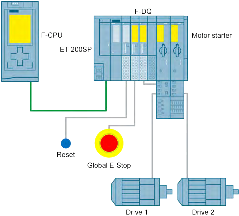
Figure 3-18 Emergency stop shutdown to SIL 3 or PL e with fail-safe digital output module and fail-safe motor starters in the ET 200SP system
