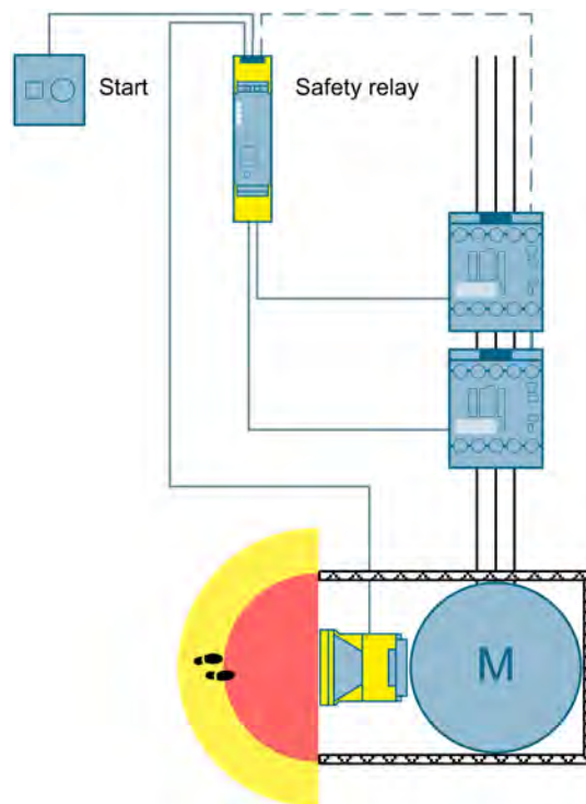
Figure 3-43 Area monitoring using a laser scanner to SIL 2 or PL d with a 3SK1 safety relay
