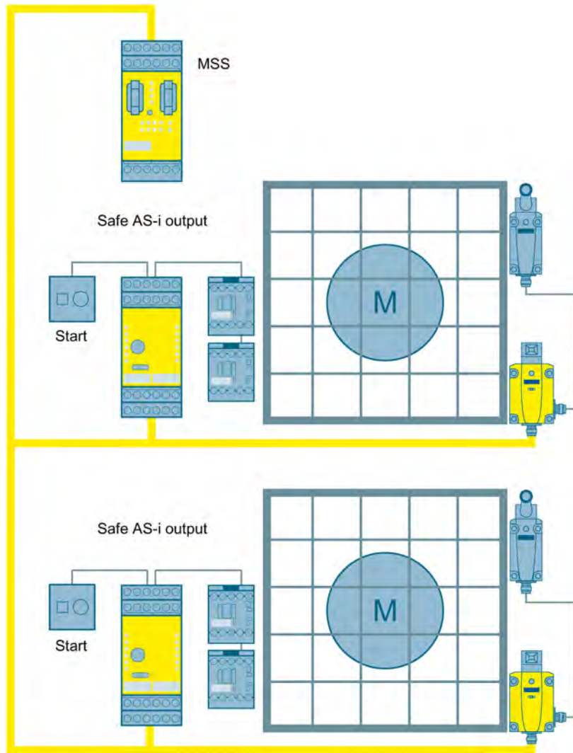
Figure 3-31 Protective door monitoring via AS-i to SIL 3 or PL e with a Modular Safety System
