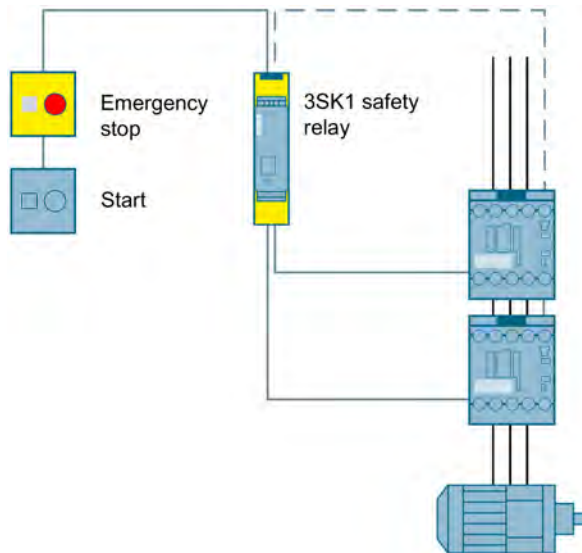
Figure 3-7 Emergency stop shutdown to SIL 3 or PL e with a 3SK1 safety relay
