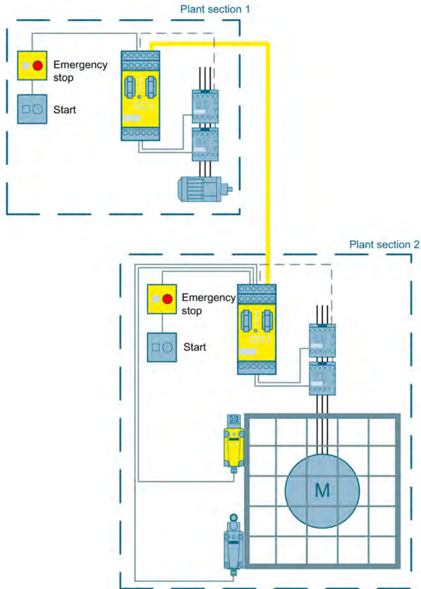
Figure 3-59 Safe slave-to-slave communication between several plant sections to SIL 3 or PL e via AS-i
