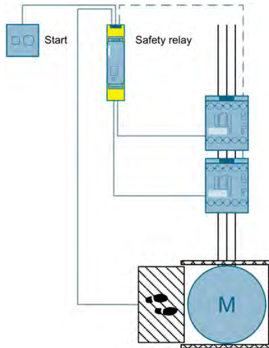
Figure 3-40 Access monitoring using a safety mat to SIL 3 or PL e with a 3SK1 safety relay
