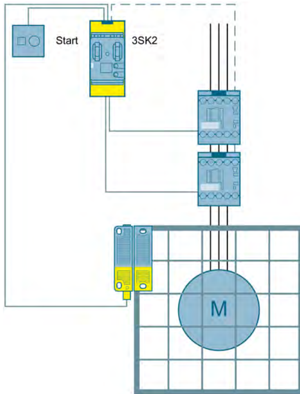
Figure 3-33 Protective door monitoring by means of RFID switch to SIL 3 or PL e with a 3SK2 safety relay
