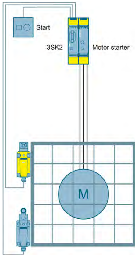
Figure 3-29 Protective door monitoring to SIL 3 or PL e with fail-safe motor starters and a 3SK2 safety relay
