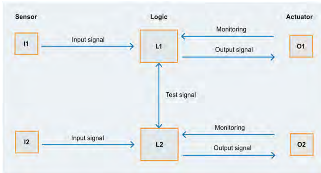
Figure 5-15 Designated architecture for Category 4
