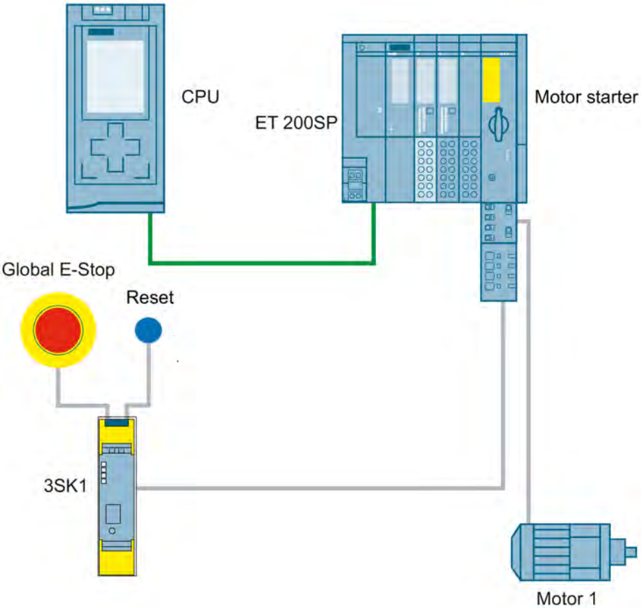
Figure 3-16 Emergency stop shutdown to SIL 3 or PL e with a fail-safe motor starter in the ET 200SP system and a 3SK1 safety relay
