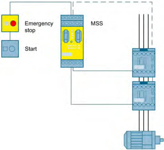
Figure 3-9 Emergency stop shutdown to SIL 3 or PL e with a modular safety system
