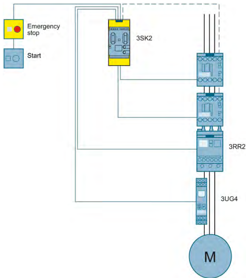
Figure 3-53 Safe current monitoring including emergency stop shutdown up to PL d with a 3SK2 safety relay and two current monitoring relays
