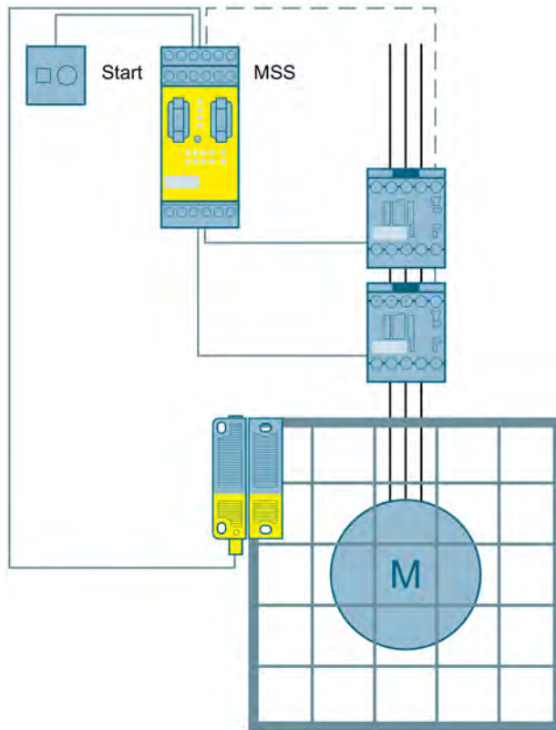
Figure 3-34 Protective door monitoring by means of RFID switch to SIL 3 or PL e with a Modular Safety System
