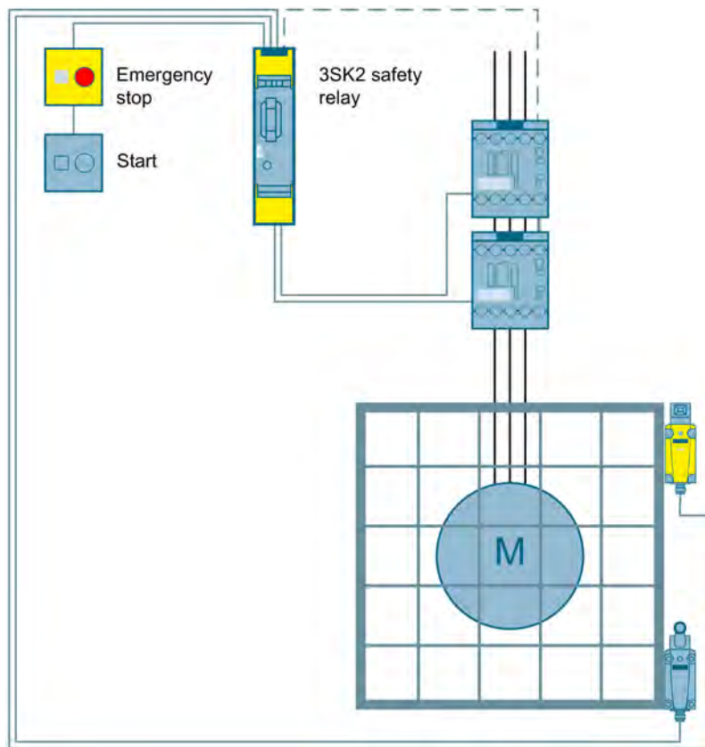
Figure 3-55 Emergency stop monitoring and protective door monitoring to SIL 3 or PL e with a 3SK2 safety relay
