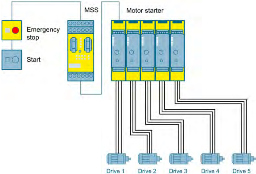
Figure 3-12 Emergency stop shutdown to SIL 3 or PL e with fail-safe motor starters and a modular safety system
