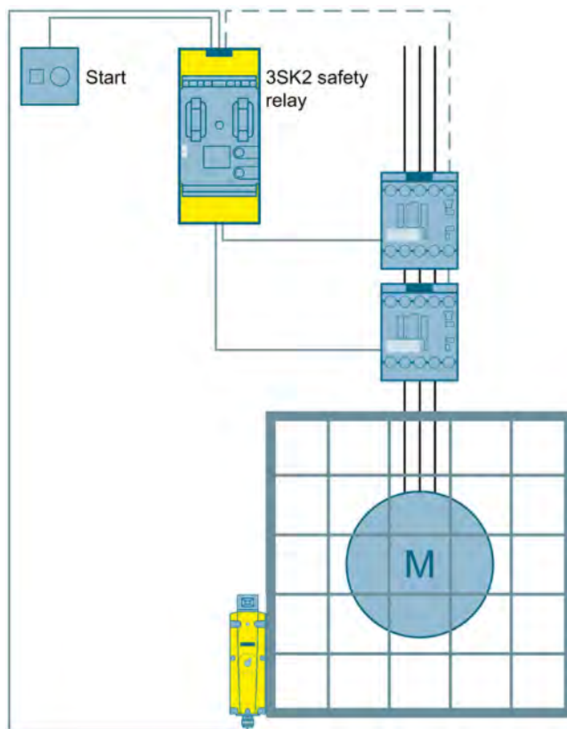
Figure 3-35 Protective door monitoring with tumbler to SIL 2 or PL d with a 3SK2 safety relay
