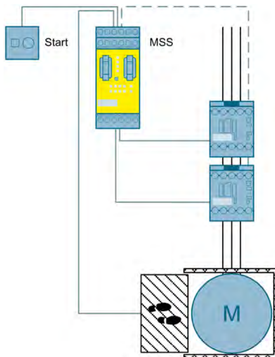
Figure 3-42 Access monitoring using a safety mat to SIL 3 or PL e with a Modular Safety System
