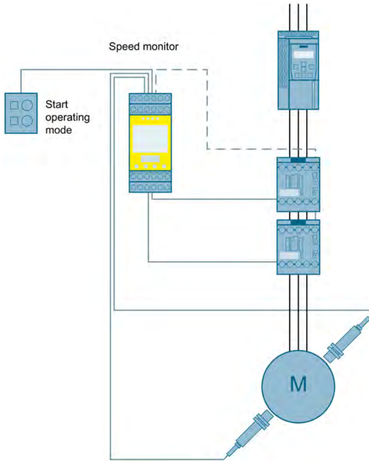
Figure 3-46 Safe speed monitoring to SIL 3 or PL e with a speed monitor
