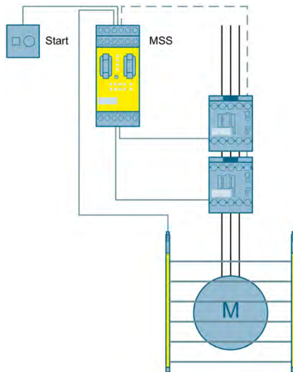
Figure 3-39 Access monitoring using a light curtain to SIL 3 or PL e with a Modular Safety System
