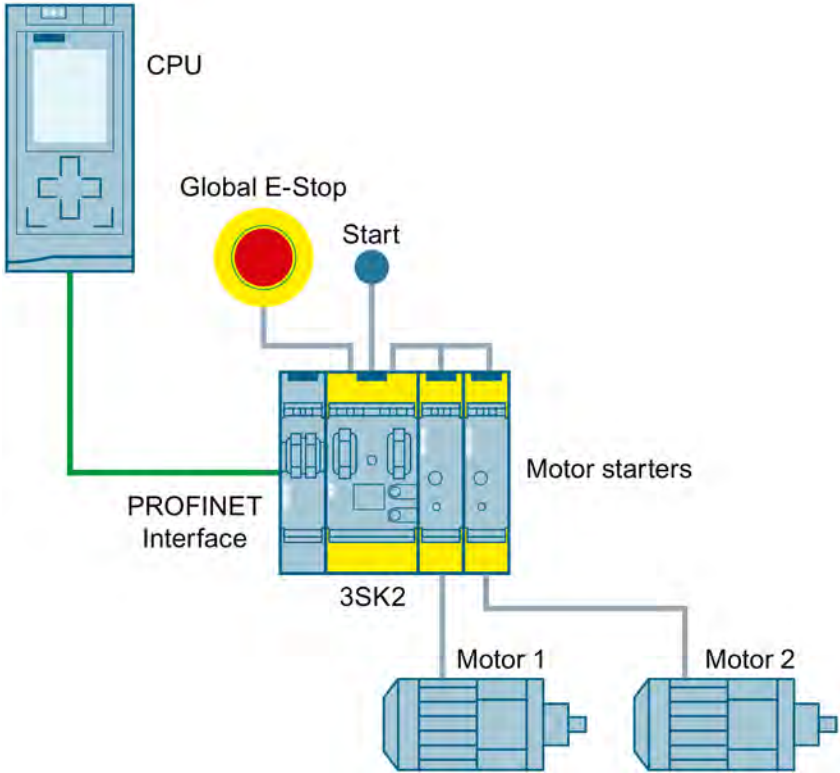
Figure 3-20 Emergency stop shutdown up to SIL 3 or PL e via 3SK2 safety relay with PROFINET connection and fail-safe motor starters
