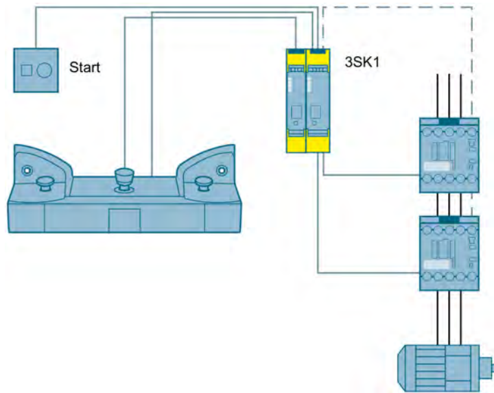
Figure 3-50 Two-hand operation to SIL 3 or PL e with a 3SK1 safety relay
