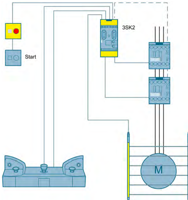
Figure 3-57 Access monitoring using a light curtain with two-hand operation and emergency stop to SIL 3 or PL e with a 3SK2 safety relay
