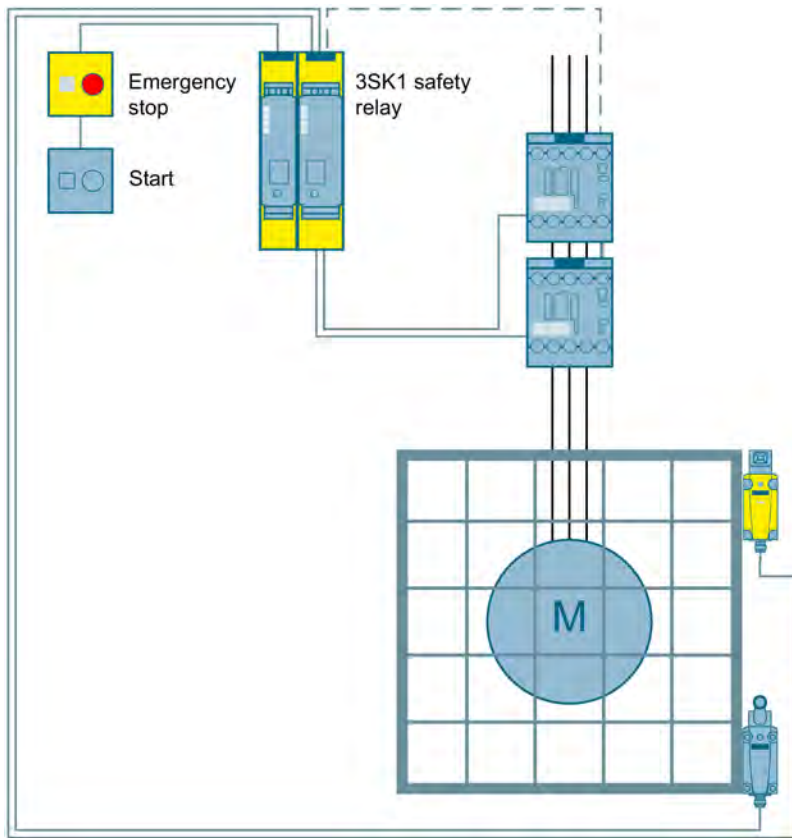
Figure 3-54 Emergency stop monitoring and protective door monitoring to SIL 3 or PL e with a 3SK1 safety relay
