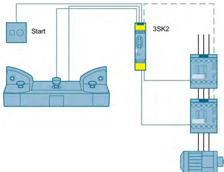
Figure 3-51 Two-hand operation to SIL 3 or PL e with a 3SK2 safety relay
