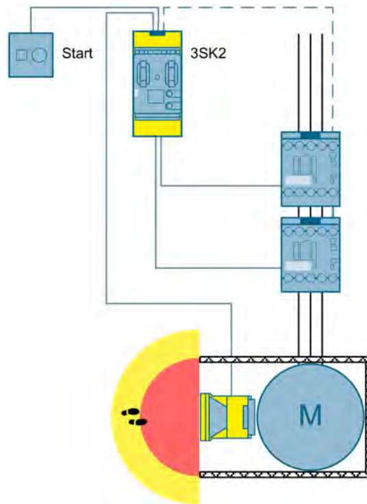
Figure 3-44 Area monitoring using a laser scanner to SIL 2 or PL d with a 3SK2 safety relay
