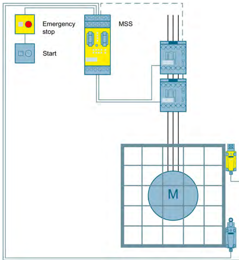
Figure 3-56 Emergency stop monitoring and protective door monitoring to SIL 3 or PL e with a Modular Safety System
