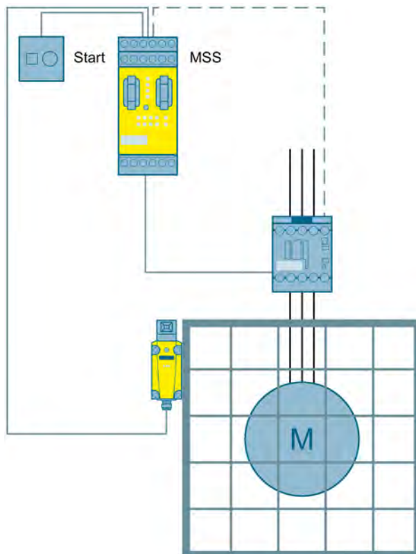
Figure 3-24 Protective door monitoring to SIL 1 or PL c with a Modular Safety System
