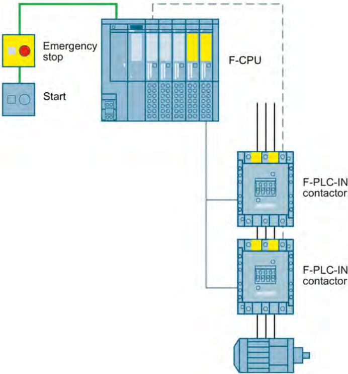
Figure 3-15 Emergency stop shutdown to SIL 3 or PL e with contactors with F-PLC-IN and fail-safe controller
