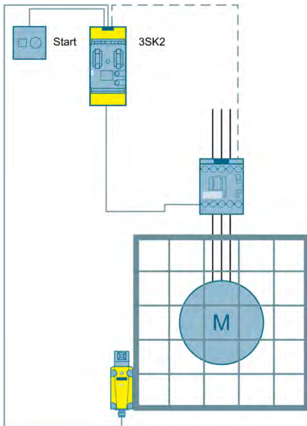
Figure 3-23 Protective door monitoring to SIL 1 or PL c with a 3SK2 safety relay
