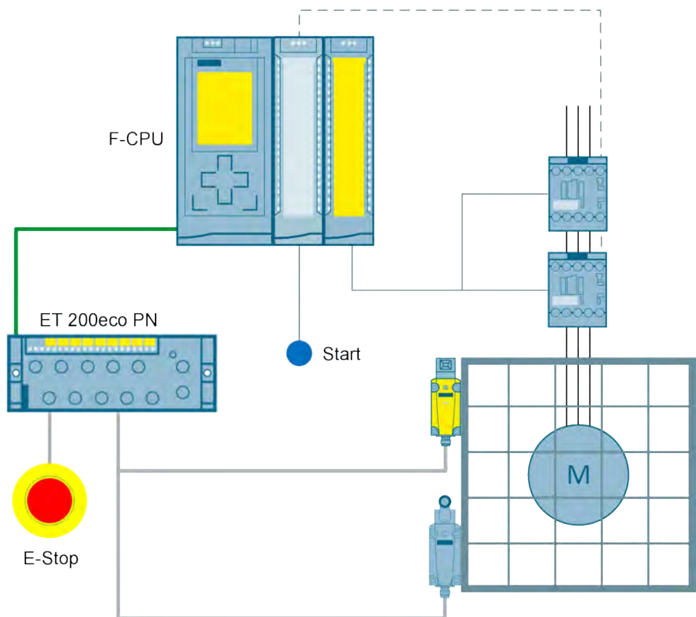
Figure 3-62 Emergency stop shutdown and protective door monitoring up to SIL 3 or PL e via ET 200eco PN and F-CPU
