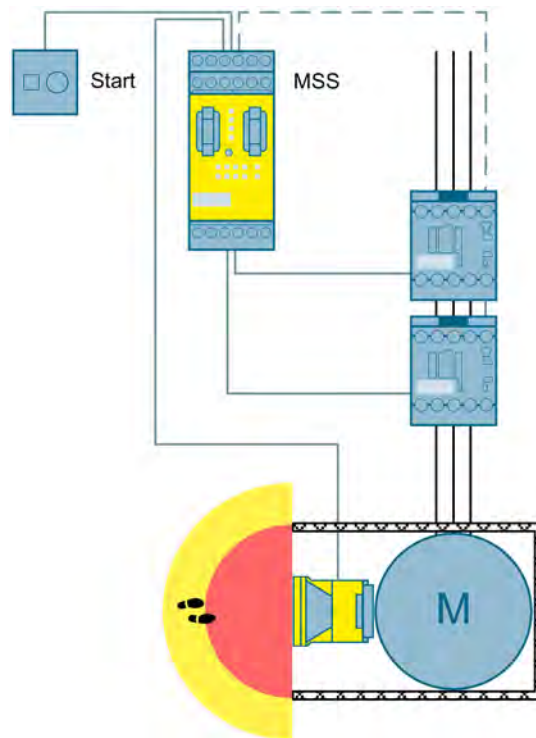
Figure 3-45 Area monitoring using a laser scanner to SIL 2 or PL d with a Modular Safety System
