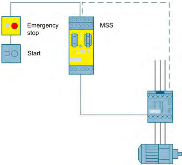
Figure 3-4 Emergency stop shutdown to SIL 1 or PL c with a Modular Safety System
