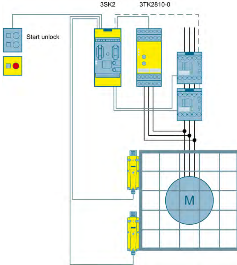
Figure 3-48 Safe standstill monitoring including protective door tumbler to SIL 3 or PL e with a 3SK2 safety relay
