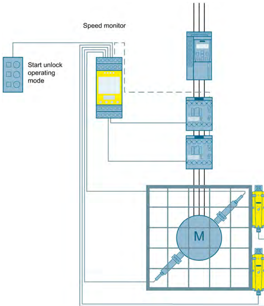
Figure 3-49 Safe speed monitoring, protective door monitoring and tumbler monitoring to SIL 3 or PL e with a speed monitor
