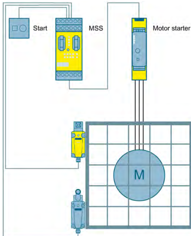
Figure 3-30 Protective door monitoring to SIL 3 or PL e with a fail-safe motor starter and a modular safety system
