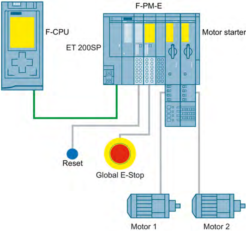
Figure 3-19 Emergency stop shutdown to SIL 3 or PL e with fail-safe power module and fail-safe motor starters in the ET 200SP system
