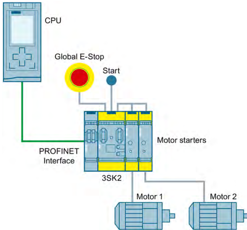
Figure 3-21 Emergency stop group shutdown up to SIL 3 or PL e via 3SK2 safety relay with PROFINET connection and fail-safe motor starters
