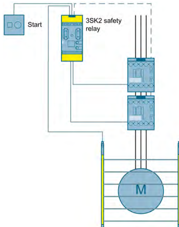
Figure 3-38 Access monitoring using a light curtain to SIL 3 or PL e with a 3SK2 safety relay
