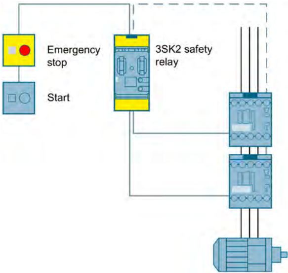
Figure 3-8 Emergency stop shutdown to SIL 3 or PL e with a 3SK2 safety relay
