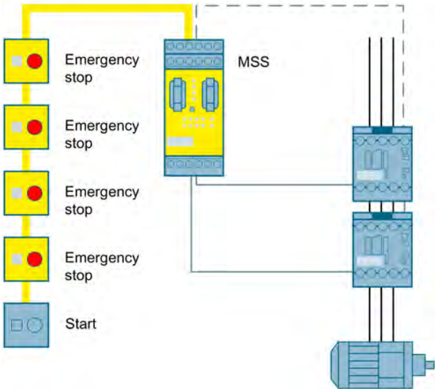
Figure 3-13 Emergency stop shutdown via AS-i to SIL 3 or PL e with a Modular Safety System
