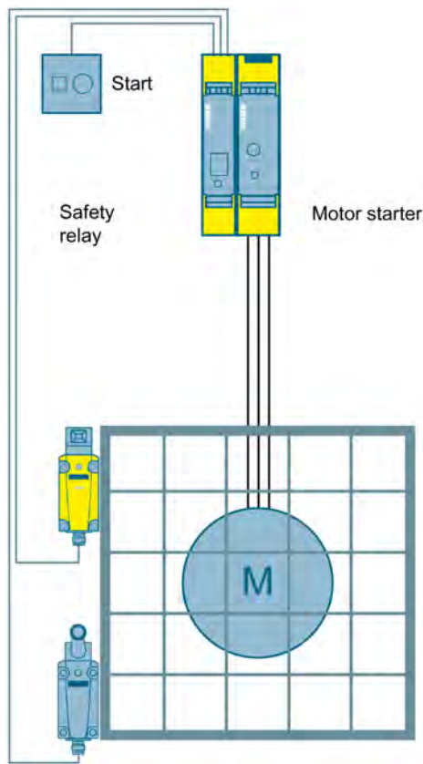
Figure 3-28 Protective door monitoring to SIL 3 or PL e with a fail-safe motor starter and a 3SK1 safety relay
