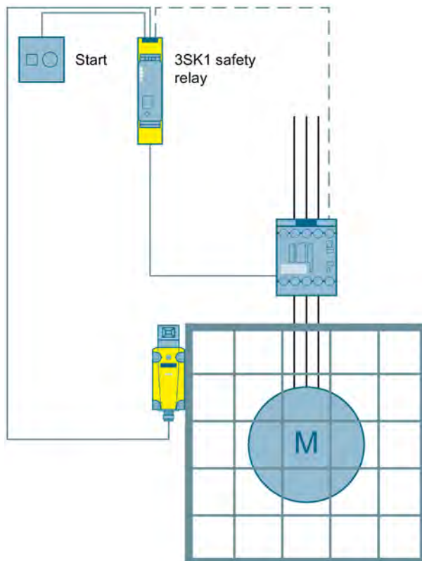
Figure 3-22 Protective door monitoring to SIL 1 or PL c with a 3SK1 safety relay
