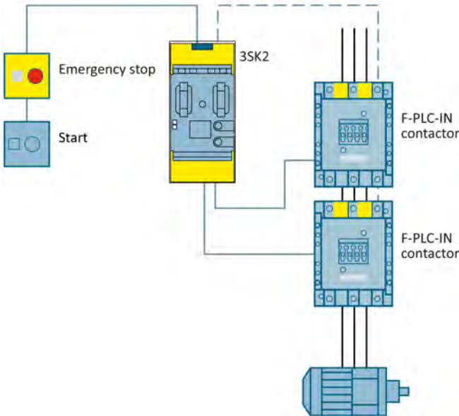
Figure 3-14 Emergency stop shutdown to SIL 3 or PL e with contactors with F-PLC-IN and 3SK2 safety relay
