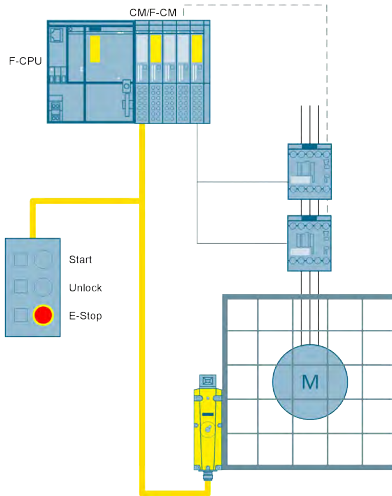
Figure 3-61 Emergency stop shutdown up to SIL 3 or PL e and protective door monitoring with tumbler up to SIL 2 or PL d via AS-i ET 200SP Master
