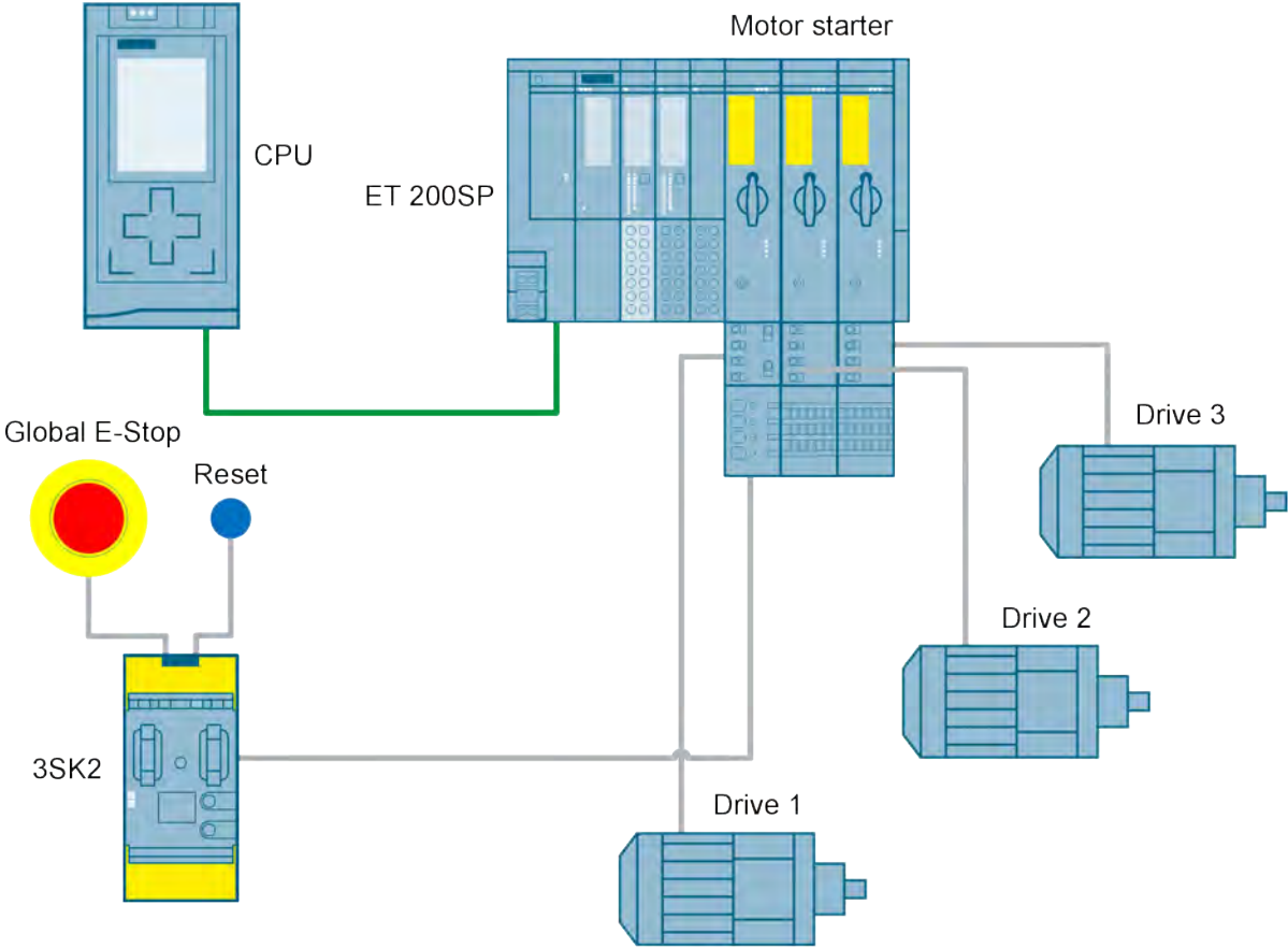
Figure 3-17 Emergency stop shutdown to SIL 3 or PL e with fail-safe motor starters in the ET 200SP system and a 3SK2 safety relay
