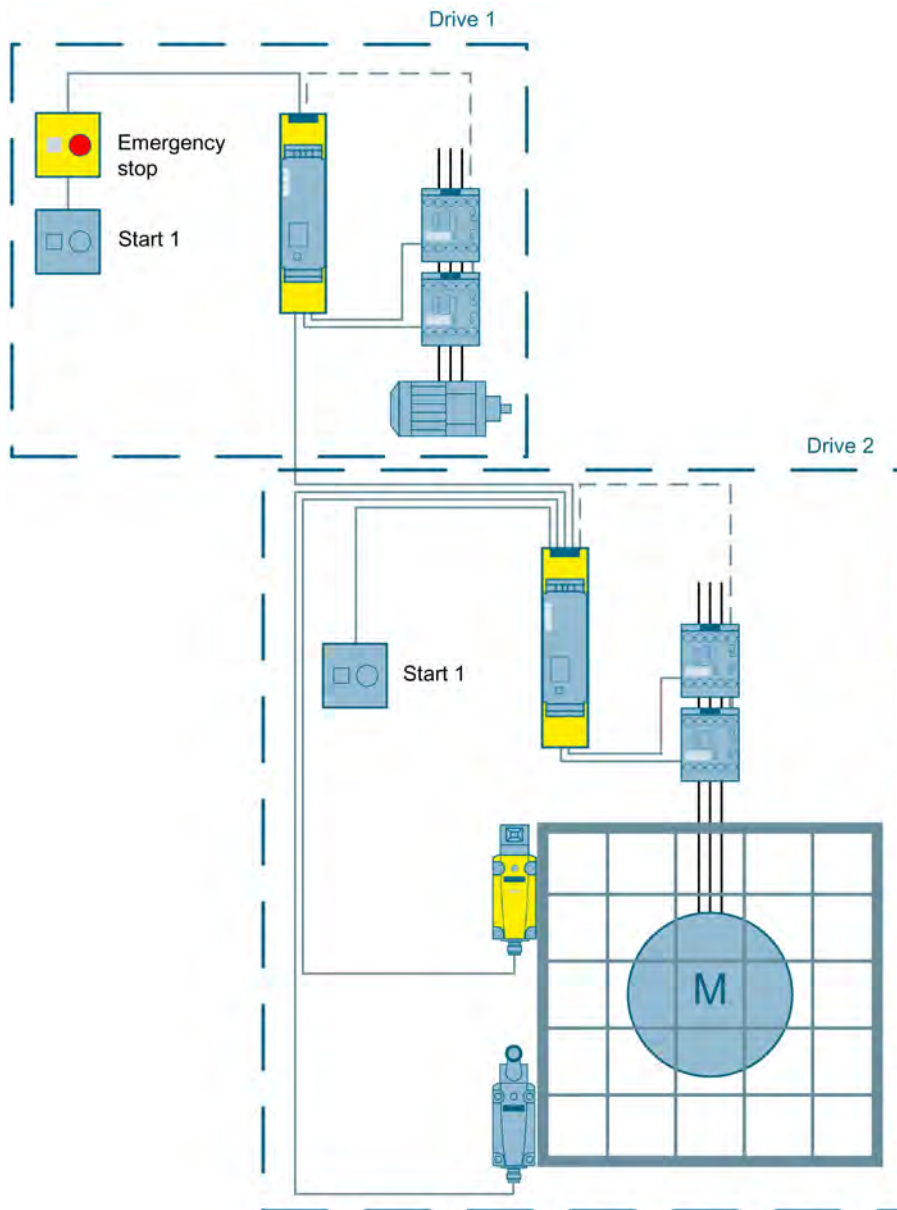
Figure 3-58 Cascading of 3SK1 safety relays to SIL 3 or PL e
