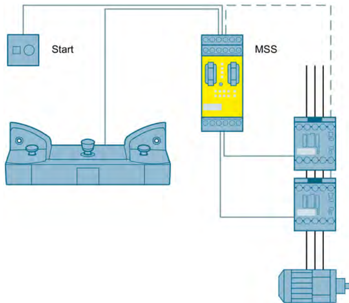
Figure 3-52 Two-hand operation to SIL 3 or PL e with a Modular Safety System
