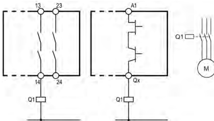
Figure 2-1 PL e acc. to ISO 13849-1, or SIL CL 1 acc. to IEC 62061
