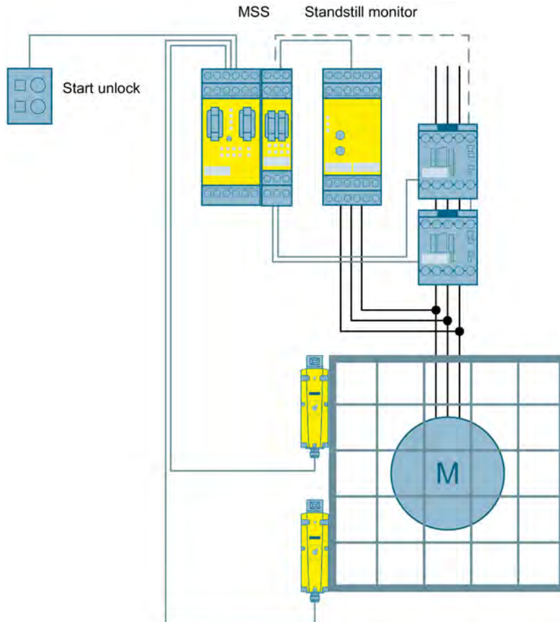
Figure 3-47 Safe standstill monitoring including protective door tumbler to SIL 3 or PL e with a Modular Safety System
