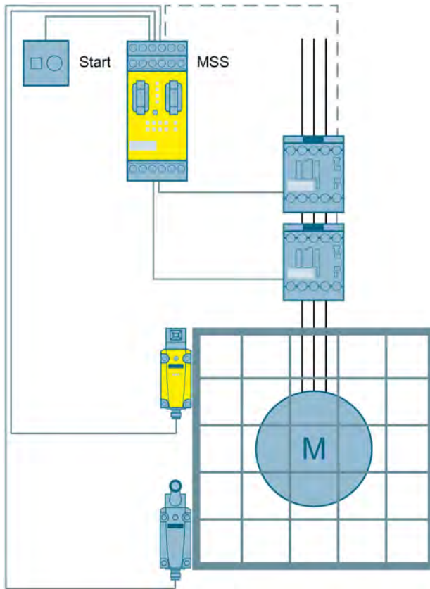
Figure 3-27 Protective door monitoring to SIL 3 or PL e with a Modular Safety System
