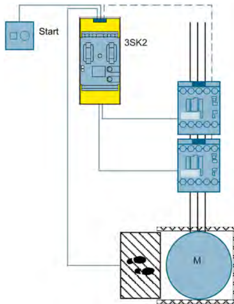
Figure 3-41 Access monitoring using a safety mat to SIL 3 or PL e with a 3SK2 safety relay
