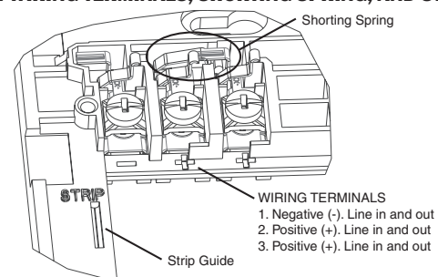
FIGURE 5. WIRING TERMINALS, SHORTING SPRING, AND STRIP GUIDE
